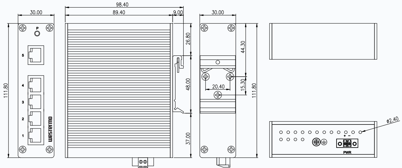
Dimensional drawing
